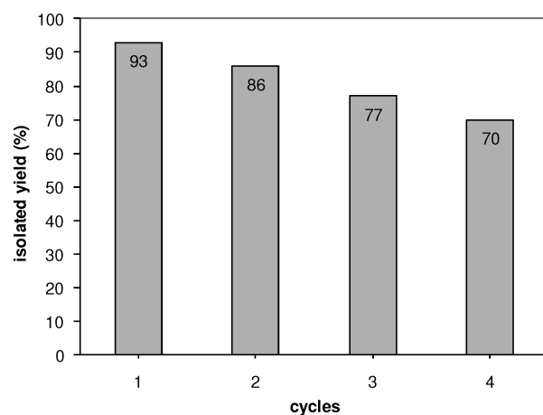
Figure 7. Recycling of the CuNPs/C in the synthesis of the triazole 3ga .
