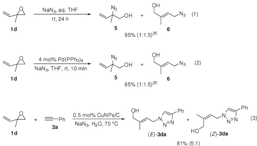
Scheme 5. Azidolysis and Domino Azidolysis–Cycloaddition of Epoxide 1d
