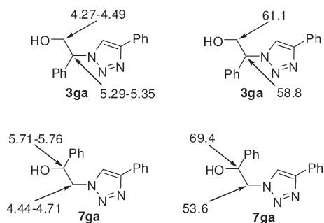
Scheme 6. Computer-Estimated 1 H and 13 C NMR Chemical Shifts (in ppm) for 3ga and 7ga
